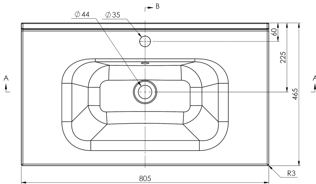
Bottom view
